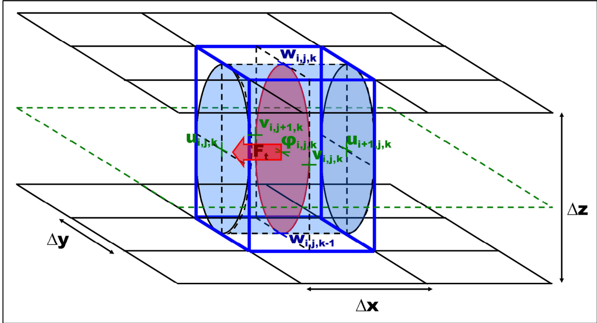
Figure 13: Staggered Grid & Control Volume. The diagram displays staggered horizontal grids at the z_w (N, N+1) levels (black lines), the z_p (N) level (green dashed plane), the actuator disc (red surface), the “smeared” actuator cylinder (light blue volume), the numerical control volume (heavy blue solid lines) and its median
