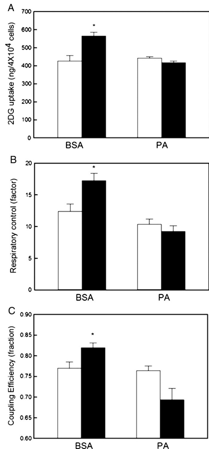
Fig. 6. Palmitate annuls insulin sensitivity of mitochondrial function. L6 myoblasts were exposed to BSA-conjugated palmitate (PA) or BSA as described in Section 2.2. 2-Deoxyglucose (2-DG) uptake (panel A), cell respiratory control (panel B), and coupling efficiency (panel C) were measured following incubation without (white bars) or with 100 nM insulin (black bars). The data shown are means \pm SEM of 5 independent experiments. The asterisks indicate statistical significance between insulin-exposed and control cells ( P < 0.05 ).
