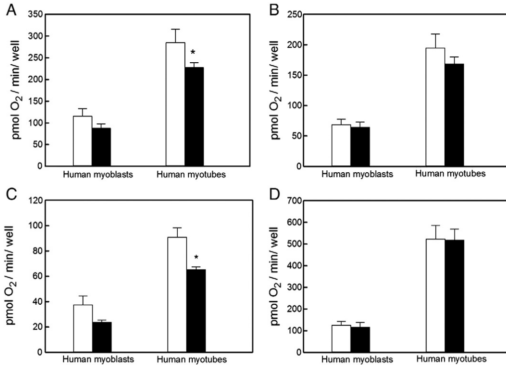
Fig. 4. Effect of insulin on absolute oxygen consumption. The basal mitochondrial respiratory rate (panel A), the oligomycin-sensitive rate (ATP turnover, panel B), the oligomycin-resistant rate (proton leak, panel C), and the FCCP-stimulated rate (maximum respiration, panel D) were expressed as total oxygen consumed per minute per XF24 well, and were calculated for human muscle cells incubated without (white bars) or with 100 nM insulin (black bars). The data shown are means \pm SEM of 3–6 independent experiments. Because of density variation between myoblasts and myotubes, only internal comparisons \pm insulin were tested statistically – the asterisks indicate significant differences ( P < 0.05 ).
