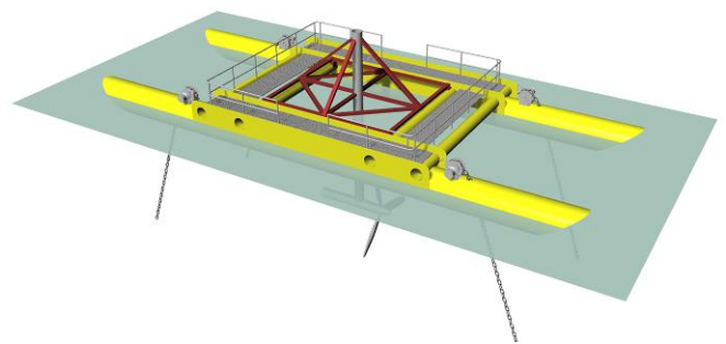
Figure 1. Prototype of the MTG device.
