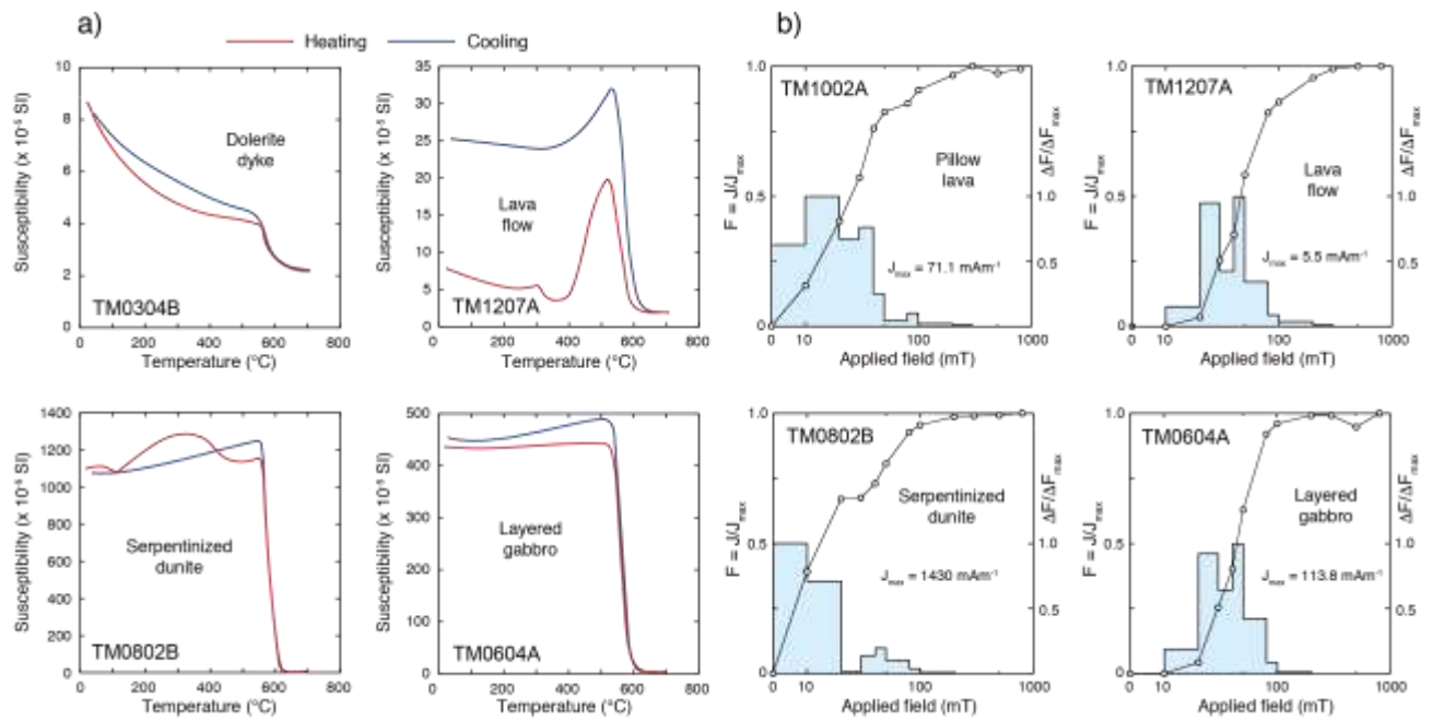
Fig. 3. Representative examples of (a) the variation of low field magnetic susceptibility with temperature and (b) isothermal remanent magnetization acquisition curves for rocks from the Thetford Mines ophiolite.
