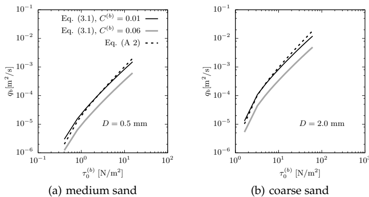
Figure 10. Comparison between bedload predicted by q_b = f(u_{s0}) (eq. A 2) and q_b = f(u_0) (eq. 3.1) for two values of C^{(b)} and for two different particle diameters.
