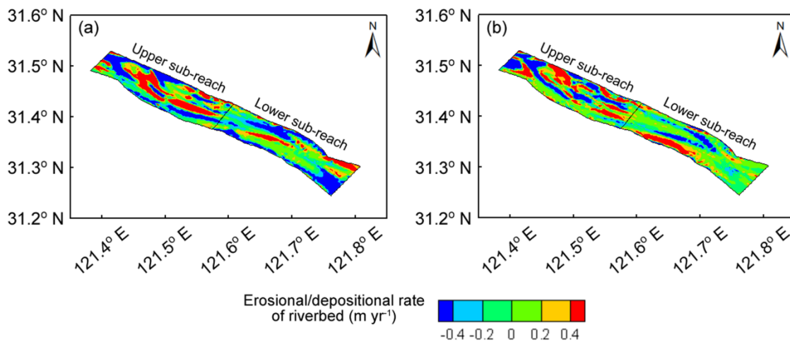
Figure S6. Plan distributions of riverbed erosion/deposition rates in the South Channel during (a) 1997-2002 and (b) 2002-2007, when the multi-year average ebb partition ratios of the South Channel were 47.83 and 50.88 % and multi-year average D_{\geq 60,000} were 29 and 4 days \text{yr}^{-1} . Positive and negative values represent deposition and erosion.
