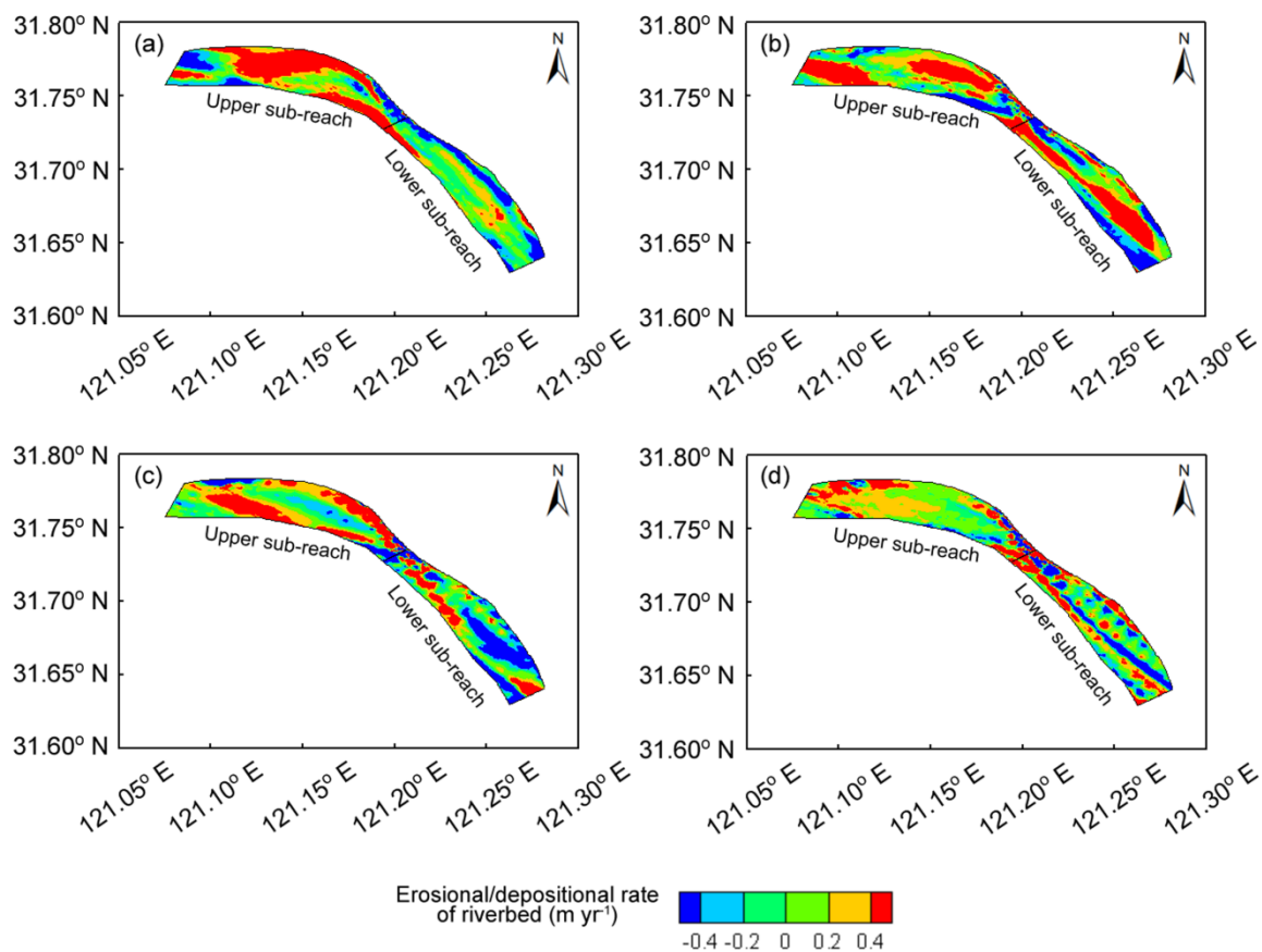
Figure S3 Plan distributions of riverbed erosion/deposition rates in the North Waterway of Baimao Shoal during (a) 1992-1999, (b) 1999-2003, (c) 2003-2007 and (d) 2007-2010. Multi-year average ebb partition ratios of the North Waterway during the latter two periods were 35.81 and 32.90 %, and multi-year average D_{\geq 60,000} values during the four periods were 31, 15, 0, and 9 days yr -1 . Positive and negative values represent deposition and erosion.
