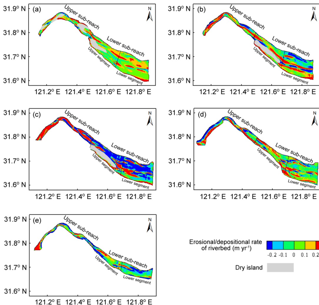
Figure S1. Plan distributions of riverbed erosion/deposition rates in the North Branch during (a) 1978-1991, (b) 1991-1998, (c) 1998-2001, (d) 2001-2007 and (e) 2007-2013, when the multi-year average ebb partition ratios of the North Branch were 0.27, 3.66, 3.66, -10.30, and -10.30 % and the multi-year average D_{\geq 60,000} values were 6, 26, 36, 3, and 5 days yr -1 . Positive and negative values represent deposition and erosion.
