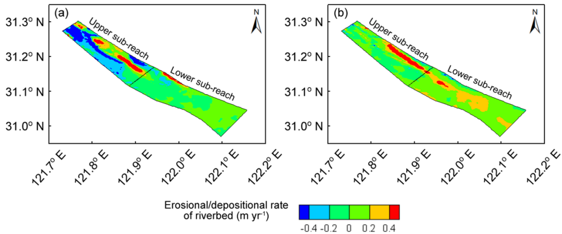
Figure S8. Plan distributions of riverbed erosion/deposition rates in the South Passage during (a) 1997-2002 and (b) 2002-2007, when the multi-year average ebb partition ratios of the South Passage were 45.17 and 51.52 % and multi-year average D_{\geq 60,000} were 29 and 4 days \text{yr}^{-1} . Positive and negative values represent deposition and erosion.
