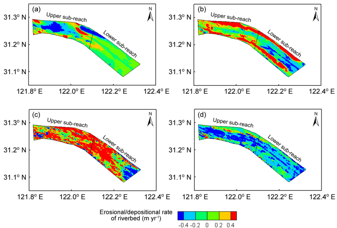
Figure S7. Plan distributions of riverbed erosion/deposition rates in the North Passage during (a) 1997-2002, (b) 2002-2006, (c) 2006-2007 and (d) 2007-2009, when multi-year average ebb partition ratios of the North Passage
