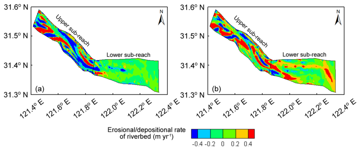
Figure S5. Plan distributions of riverbed erosion/deposition rates in the North Channel during (a) 1997-2002 and (b) 2002-2007, when the multi-year average ebb partition ratios of the North Channel were 52.17 and 49.12 % and the multi-year average D_{\geq 60,000} values were 29 and 4 days \text{yr}^{-1} . Positive and negative values represent deposition and erosion.
