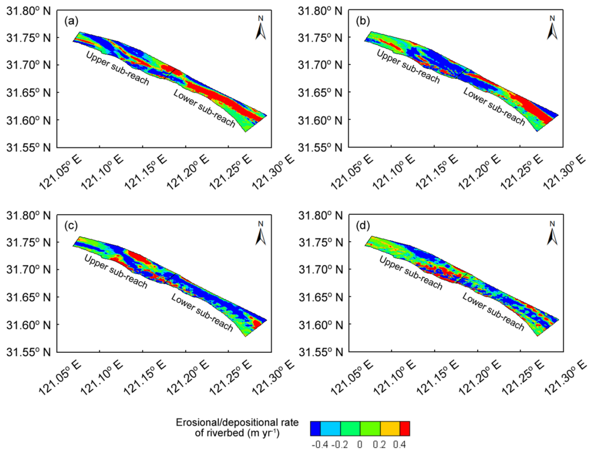
Figure S4. Plan distributions of riverbed erosion/deposition rates in the South Waterway of Baimao Shoal during (a) 1992-1999, (b) 1999-2003, (c) 2003-2007, and (d) 2007-2010. Multi-year average ebb partition ratios of the South Waterway during the latter two periods were 64.19 and 67.10 %, and multi-year average D_{\geq 60,000} values during the four periods were 31, 15, 0, and 9 days \text{yr}^{-1} . Positive and negative values represent deposition and erosion.
