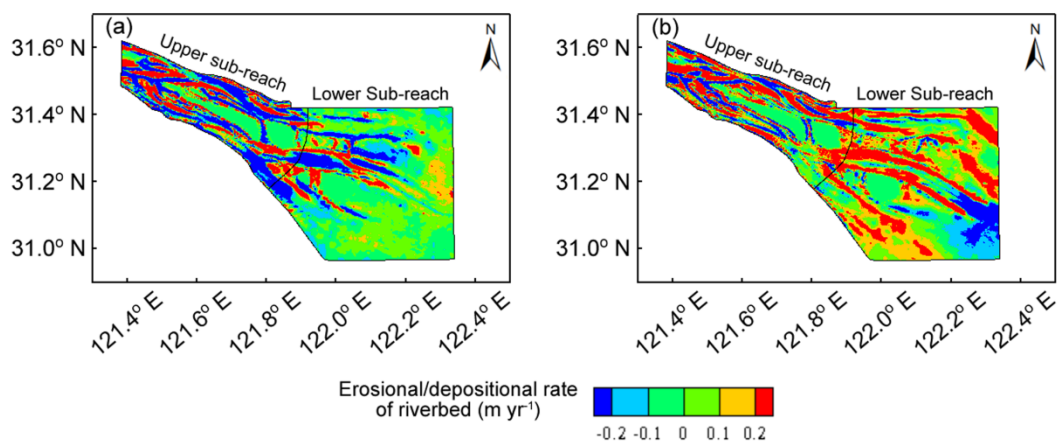
Figure S2. Plan distributions of riverbed erosion/deposition rates in the South Branch during (a) 1997-2002 and (b) 2002-2007, when the multi-year average ebb partition ratios of the South Branch were 96.34 and 110.30 % respectively and multi-year average D_{\geq 60,000} values were 29 and 4 days yr -1 . Positive and negative values represent deposition and erosion.
