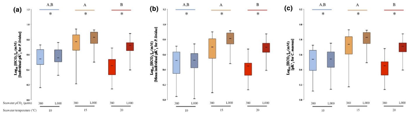
FIGURE 4 The effects of elevated seawater p\text{CO}_2 and temperature on coelomic fluid \text{Log}_{10} [\text{HCO}_3^-]_{cf} of the sea urchin P. lividus . [\text{HCO}_3^-]_{cf} determined using (a) individual values of pK'_1 for P. lividus , (b) the mean individual pK'_1 for P. lividus , and (c) pK'_1 for C. maenas . Temperature treatments are identified by blue, orange, and red colors for 10, 15, and 20°C, respectively. Ambient seawater p\text{CO}_2 ( \approx 300 \mu\text{atm} ) and elevated seawater p\text{CO}_2 ( \approx 1,000 \mu\text{atm} ) are identified by plain and hatched box plot, respectively. Capital letters indicate significant differences ( p < 0.05 ) between temperature treatments. Asterisks indicate significant differences ( p < 0.05 ) between p\text{CO}_2 treatments at the same temperature treatment
