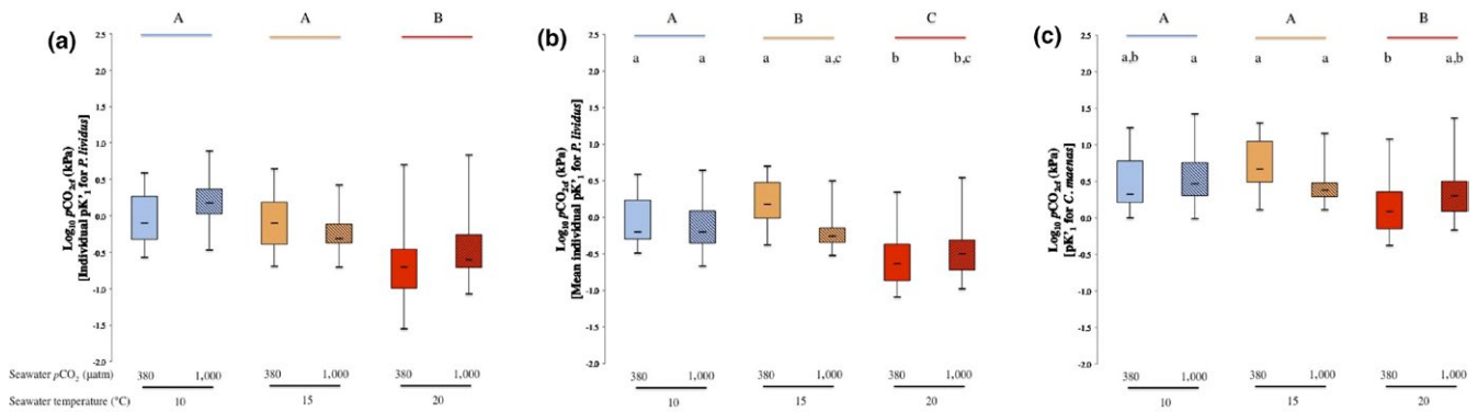
FIGURE 3 The effects of elevated seawater p\text{CO}_2 and temperature on coelomic fluid \text{Log}_{10} p\text{CO}_2 of the sea urchin P. lividus . p\text{CO}_{2cf} determined (a) using individual values of pK'_1 for P. lividus , (b) using the mean individual pK'_1 for P. lividus , and (c) using pK'_1 for Carcinus maenas . Temperature treatments are indicated by blue, orange, and red colors for 10, 15, and 20°C, respectively. Ambient seawater p\text{CO}_2 ( \approx 300 \mu\text{atm} ) and elevated seawater p\text{CO}_2 ( \approx 1,000 \mu\text{atm} ) are indicated by plain and hatched box plot, respectively. Lower case letters identify significant differences ( p < 0.05 ) between treatments. Capital letters identify significant differences ( p < 0.05 ) between temperature treatments
