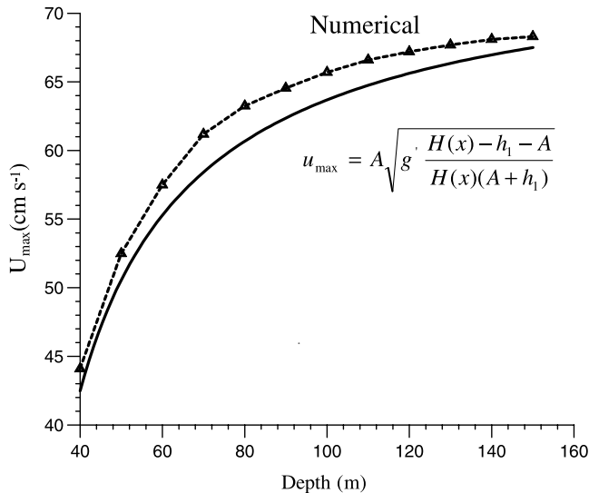
Figure 15. Numerically found dependence of maximum velocity of fluid particles at the free surface at the soliton centers, U_{\max} , on water depth (dashed line). The solid line is the function u_{1m}(H) found from the two-layer model (see equation (10)).
