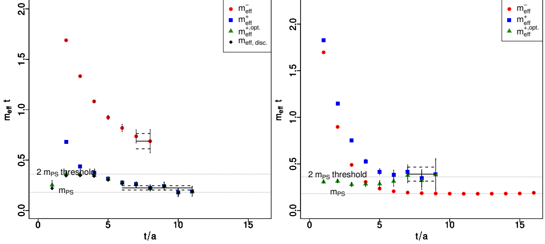
(a) iso-vector and iso-scalar scalar operator.
