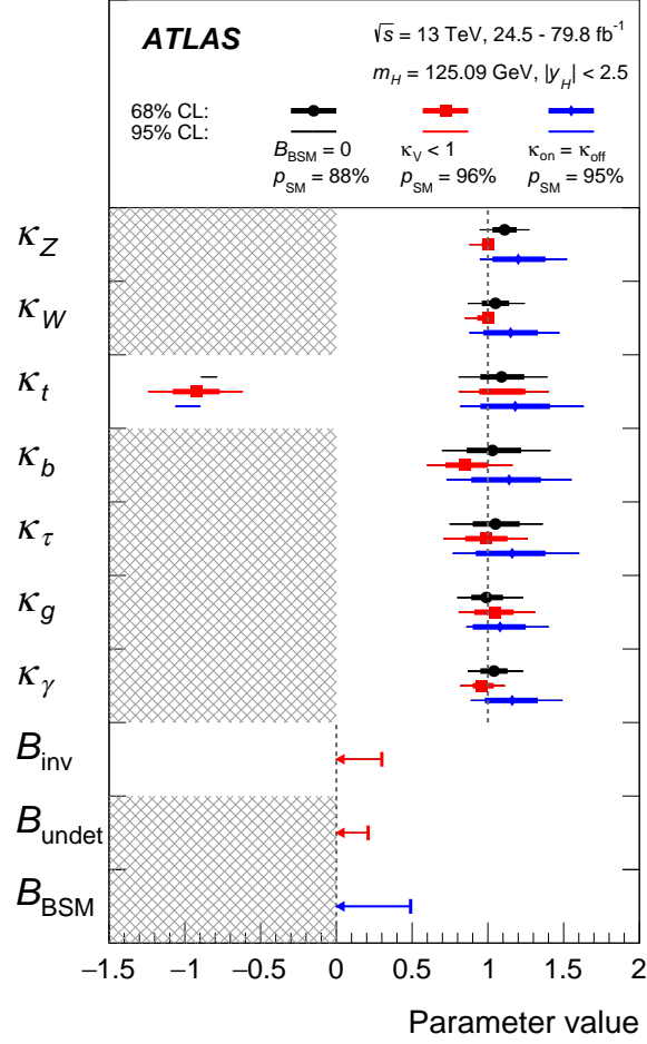
Figure 1: Best-fit values and uncertainties for Higgs boson coupling modifiers per particle type with effective photon and gluon couplings assuming no BSM contributions (black). More details can be found in [6].
