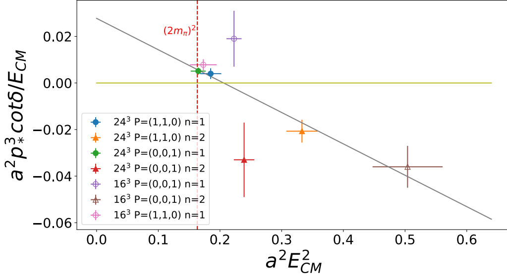
Figure 7: Plot of a^2 p_*^3 \cot \delta / E_{CM} as a function of the squared centre-of-mass energy. Points with error bars correspond to energy levels from different ensembles and/or total momenta P . A linear fit allows to determine the resonance parameters.
