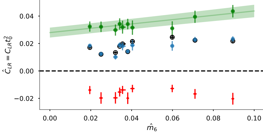
Figure 10: Fit of the C_{LR} data, the continuum prediction is shown by a green band
