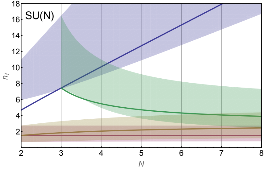
Figure 2: Perturbative (4-loops \bar{M}\bar{S} ) calculation of the conformal window for SU(N) groups in the fundamental representation (upper light-blue), two-index antisymmetric (next to the highest light-green), two-index symmetric (third window from the top light-brown) and finally the adjoint representation (bottom light-pink)[9].
