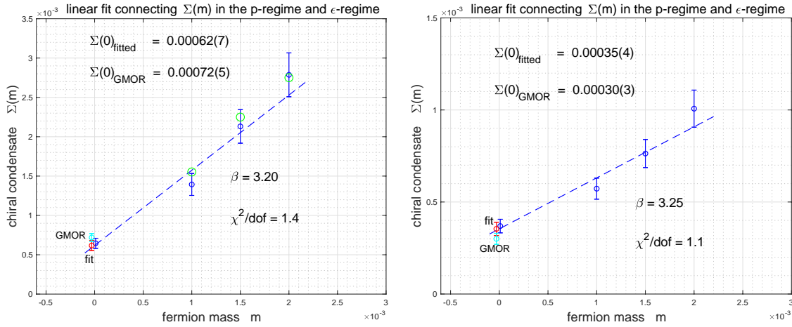
Figure 5: Comparison of the chiral condensate \Sigma(m) obtained from simulations in the \varepsilon -regime and by the GMOR relation in the p -regime for two sextet (Dirac) fermions of SU(3) gauge theory. More details can be found in [31].
