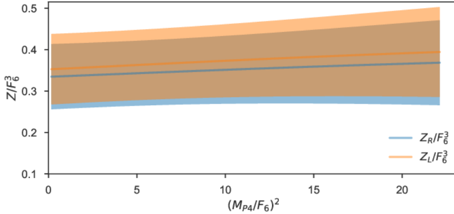
Figure 9: Chimera baryon matrix elements as a function of of the quartet mass.
