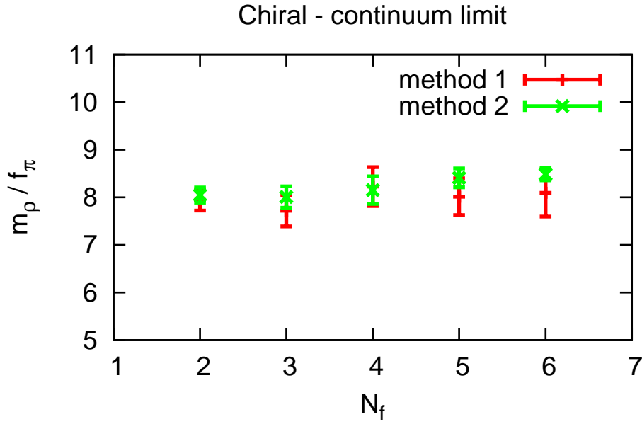
Figure 11: The ratio m_\rho / f_\pi in the chiral-continuum limit for each N_f [82].
