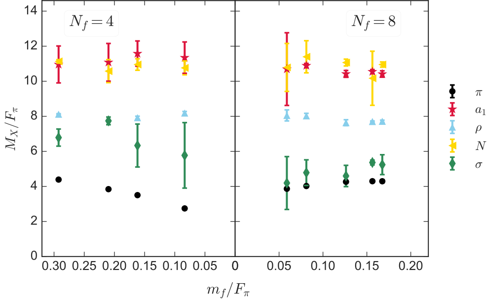
Figure 4: Comparison of the spectroscopy of SU(3) gauge theory for N_f = 4 (left) and N_f = 8 (right) fundamental fermions with. Hadron masses (vertical axis) and the fundamental fermion mass (horizontal axis) are both shown in units of the pion decay constant F_\pi ; the chiral limit m_f = 0 is at the center of the plot for both theories. The major qualitative difference between the two values of N_f is the degeneracy of the light scalar \sigma with the pions at N_f = 8 . [21]
