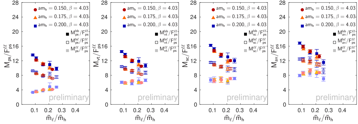
Figure 6: Low-lying connected meson spectrum obtained from light-light, heavy-light, or heavy-heavy two-point correlator functions as a function of the ratio of light over heavy flavour mass to highlight hyperscaling[45].
