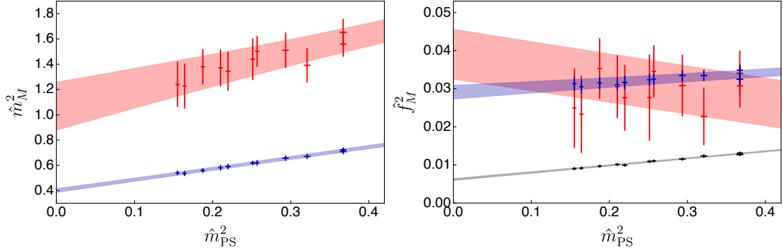
Figure 8: Continuum-extrapolated meson masses and decay constants squared as a function of the pseudo-scalar mass squared. Black, blue and red colours are for PS, V and AV mesons. The global fit results are denoted by shaded bands with their widths representing the statistical errors.
