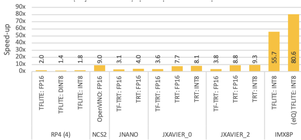
FIGURE 24. Method2: Evaluation/comparison of the optimization frameworks
