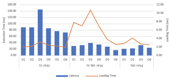
FIGURE 19. Method2: Latency evaluation/comparison of the OD models on the JNANO
