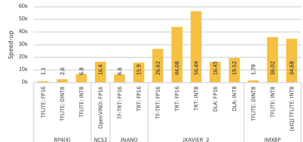
FIGURE 13. Method1: Evaluation/comparison of the optimization frameworks (average speed-up is shown)
