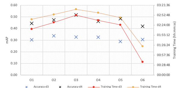
FIGURE 3. Image Classification Models: Accuracy/Training Time Plot (20 epochs)
