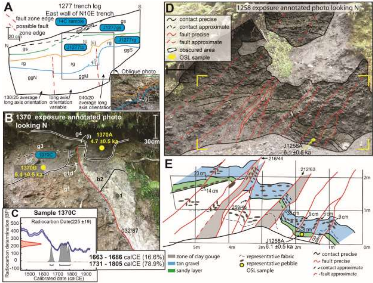
Figure 14. Observations and samples from exposures at Site 8: Styx River fan. A) Log of the east wall of the hand-dug trench 1277 with annotated photo. Photo was taken oblique to the trench wall, extent indicated on log with black box. 14C sample locations are shown in blue, parenthetical roman numerals reference positions mentioned in the text. Colours of unit contacts correspond to annotations in the photo. The central area between the dashed red lines of non-imbricated gravel is interpreted as the fault zone. Section of disorganised gravel (ggM) is interpreted as a fault zone, on either end of the trench exposure the gravel is well imbricated. It is uncertain if unit rg is faulted or simply deposited over the rough surface topography of gg, but the rough upper contact of rg suggests the unit is faulted. Upper units tc and gs are not interpreted as faulted. All three 14C samples returned modern ages. B) Exposure 1370 at Site 8, photo with annotations and sample locations. A) Solid lines are sharp contacts, dashed lines are gradational contacts. Fault is shown in red, fault strikes 032° and dips 67°E. OSL samples are shown with yellow circles, 14C sample location with blue oval. Sheared bedrock units (b1 and b2) in the hanging wall of the fault. Deformed gravel units (g1 and g2) are in the footwall and undeformed gravel (g3) and sand (g4) overlie the fault and unit b2. Units are further described in the text. B) Calibration curve for 14C sample 1370C, calibrated age is 1663-1805 CE (OxCal v4.4.4 Bronk Ramsey, 2021; Atmospheric data from Hogg et al., 2020). C and D) Exposure 1258 at Site 8, annotated photo and gridded outcrop log. The yellow circle indicates the location of OSL sample 1258A. Distinctive tan gravel unit and underlying thin sand are shown in the annotated log. Numbers in the annotated log indicate either apparent vertical displacement of a marker bed (cm), or the strike/dip of a fault.
