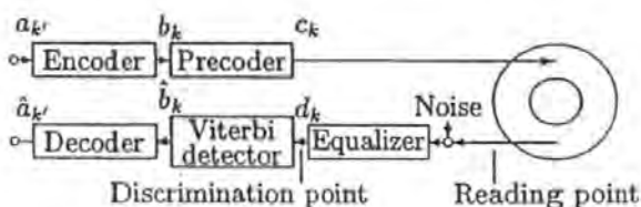
Fig. 1. Block diagram.
