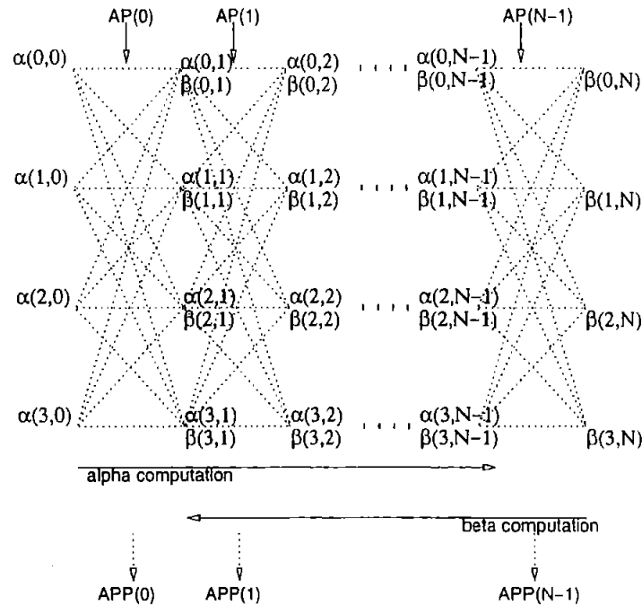
Figure 3.4: BCJR Trellis for New PR4 Trellis
