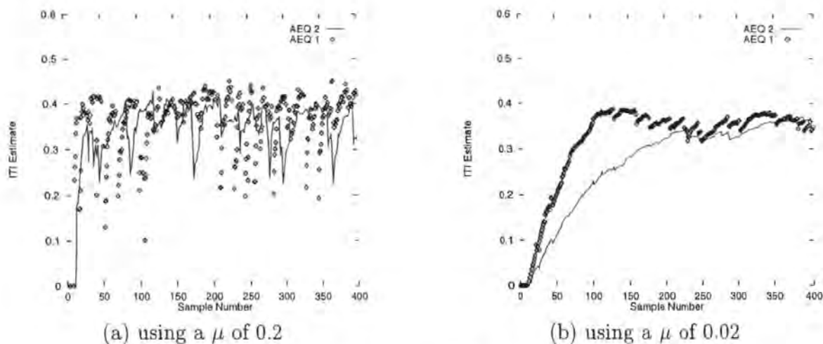
Figure 5.4: Estimated \alpha for an SNR of 25dB, Ideal \alpha = 0.4
