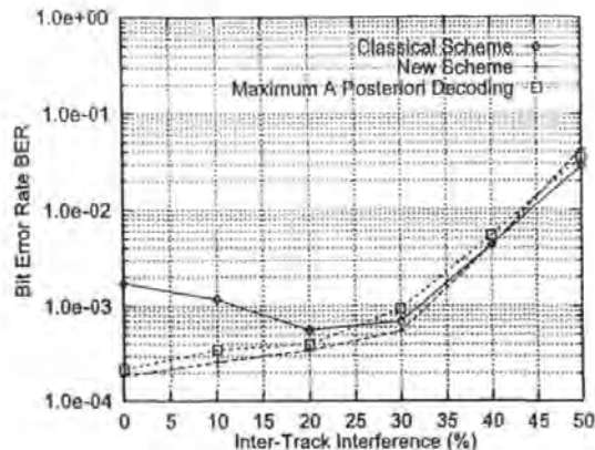
Fig. 4. Comparison of New Decoding Scheme with a Classical scheme
