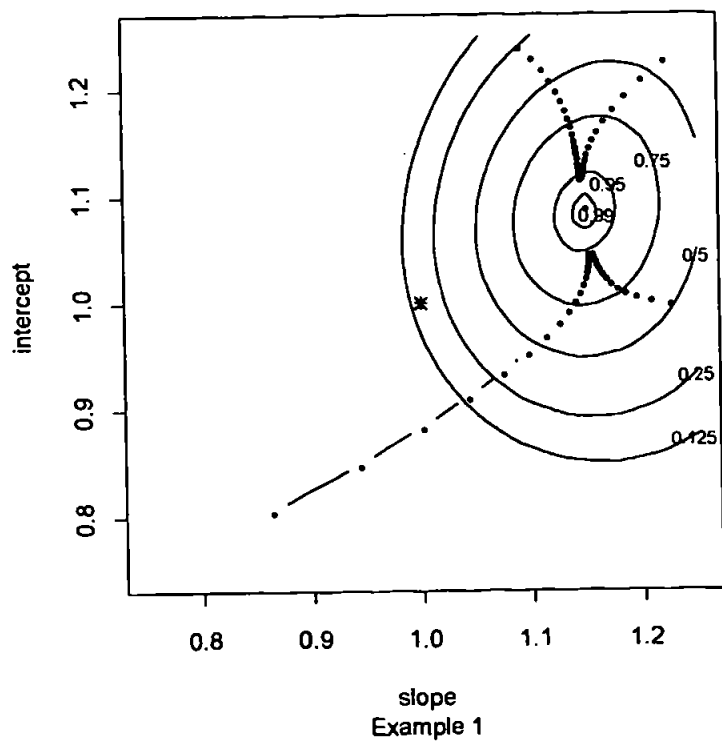
Likelihood Functions and Iteration Paths for two simulated data sets.
