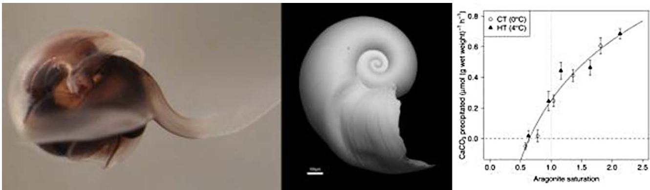
Figure 7.2. Left: A living pteropod from the Arctic (image Vicky Peck, BAS). Centre: The shell of a juvenile pteropod from the South Atlantic. Right: Data from laboratory culture experiments on shell growth rate of Limacina helicina incubated under aragonite saturation states equivalent to those seen in the Arctic at present day (ca 2.0) to the year 2100 (<1.0), from [41] .
